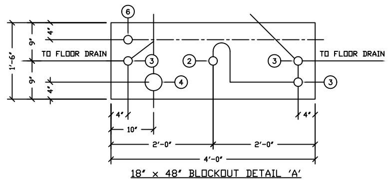
FLOOR DRAIN BLOCKOUTS & BELOW FLOOR PIPING
