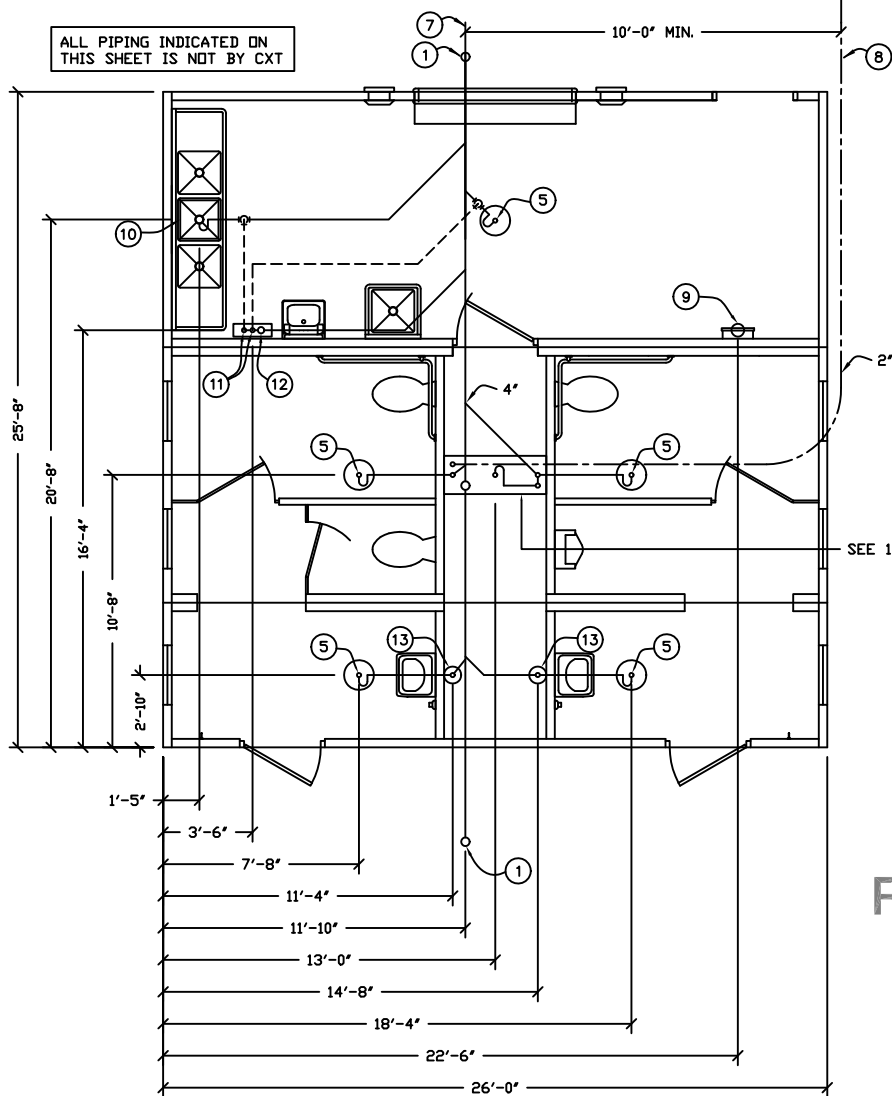
FLOOR DRAIN BLOCKOUTS & BELOW FLOOR PIPING
