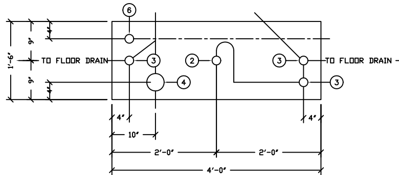
18" x 48" BLOCKOUT DETAIL
