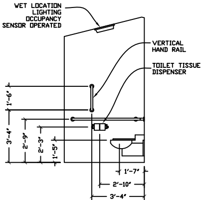
SECTION VIEW A-A - RIGHT HAND RESTROOM
