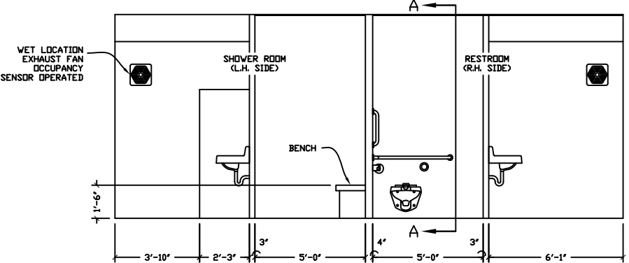
INTERIOR ELEVATION
