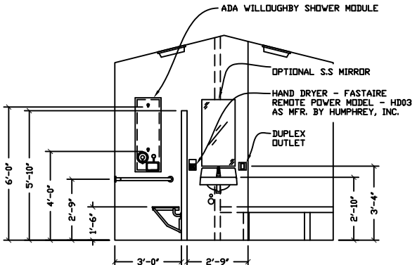
INTERIOR ELEVATION - LEFT HAND SHOWER
