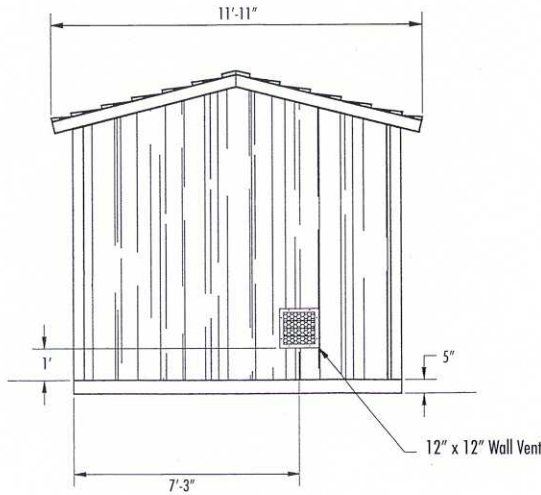
Back Elevation
